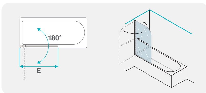
Parete per vasca / bath tub wall / paroi baignoire / badewannewand pared bañera
