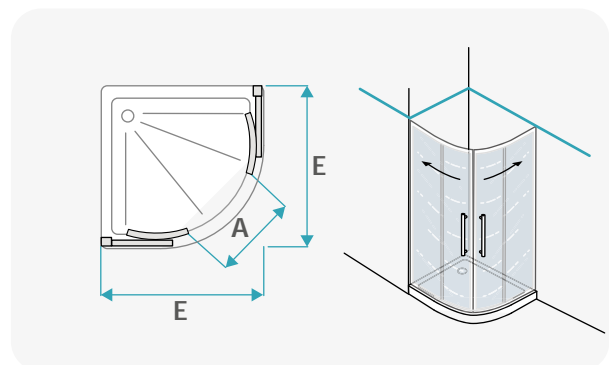
Porta scorrevole semicircolare / semicircular sliding door / coulissante semi-circulaire / halbkreise schiebetür / puerta corredera semicircular
